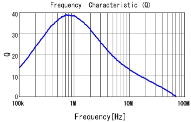
DFE201612E-1R0M Q
