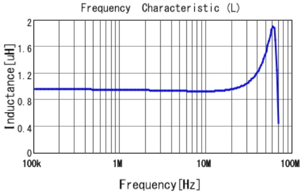
DFE201612E-1R0M L
