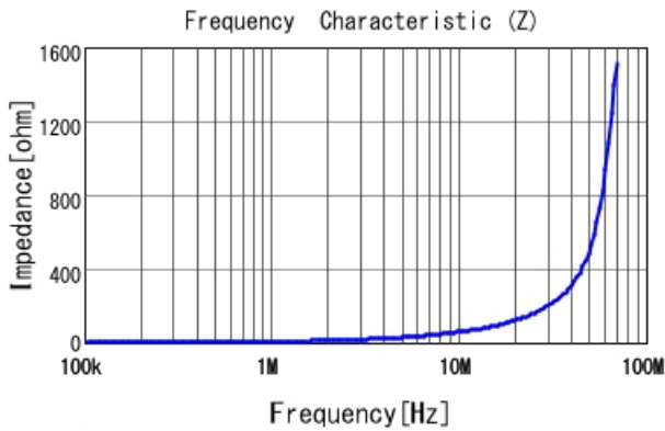
DFE201612E-1R0M |Z|
