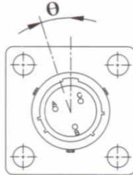
Alternate position of insert with socket contacts ( \theta counterclockwise)
