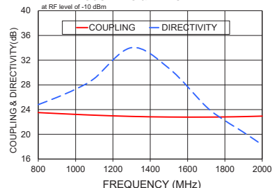
ZNDC-23-2G-S+ COUPLING & DIRECTIVITY
