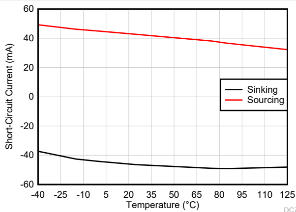
Figure 6-35. Short-Circuit Current vs Temperature
