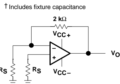
Figure 3. Noise-Voltage Test Circuit
