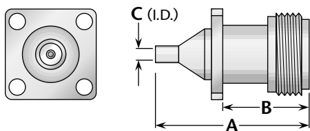
Figure 2 (One-Step cable attachment—see page 74 for details)
