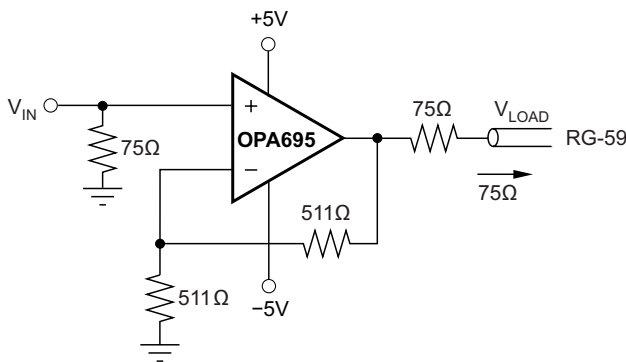
Gain 2V/V Video Line Driver
