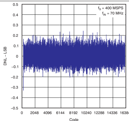
Figure 15. Differential Nonlinearity
