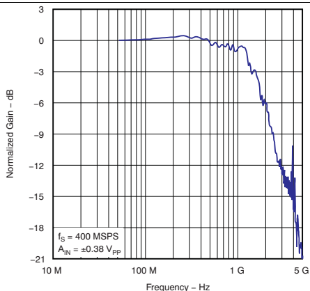
Figure 14. Normalized Gain Response vs Input Frequency
